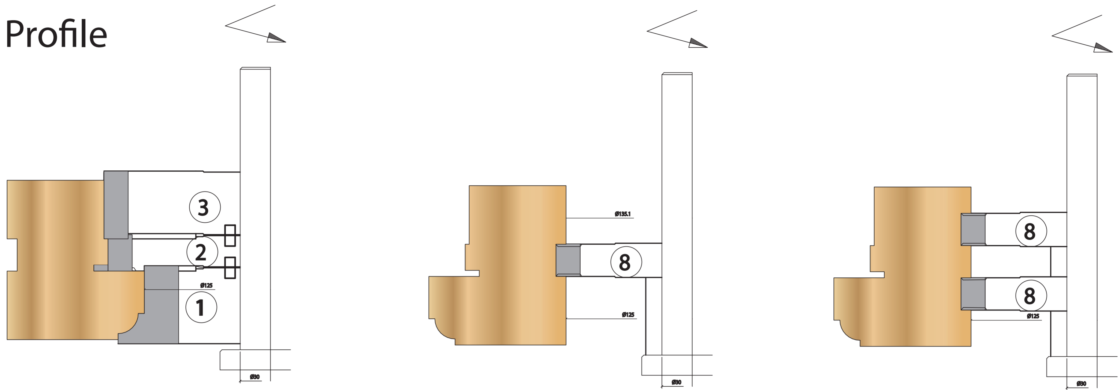
Tenon Frame
