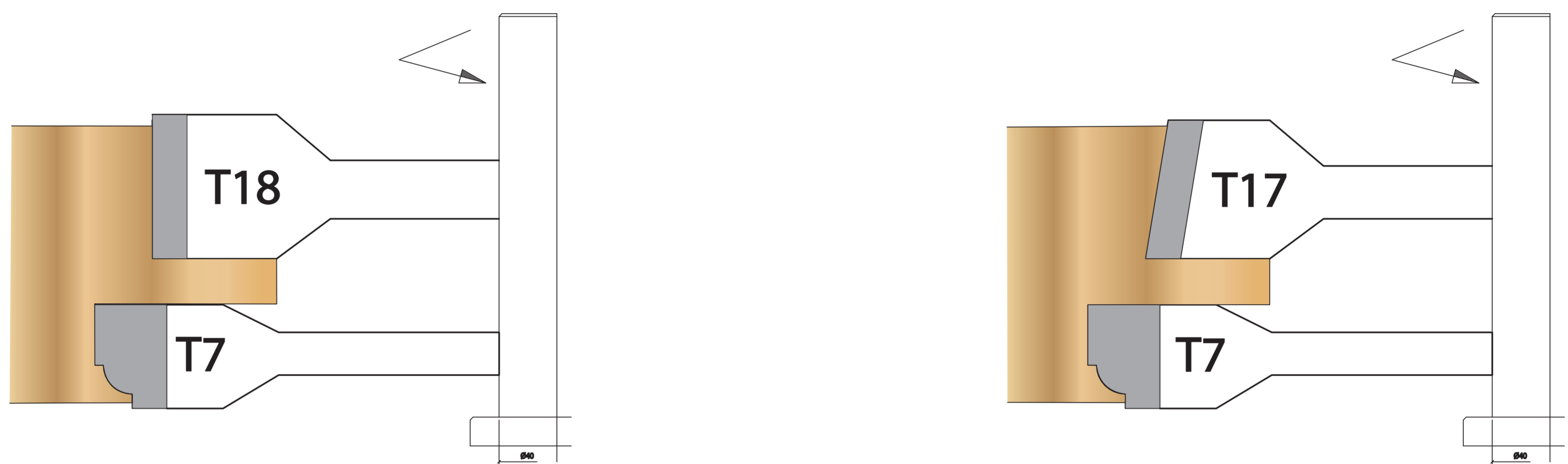
Tenon Frame
