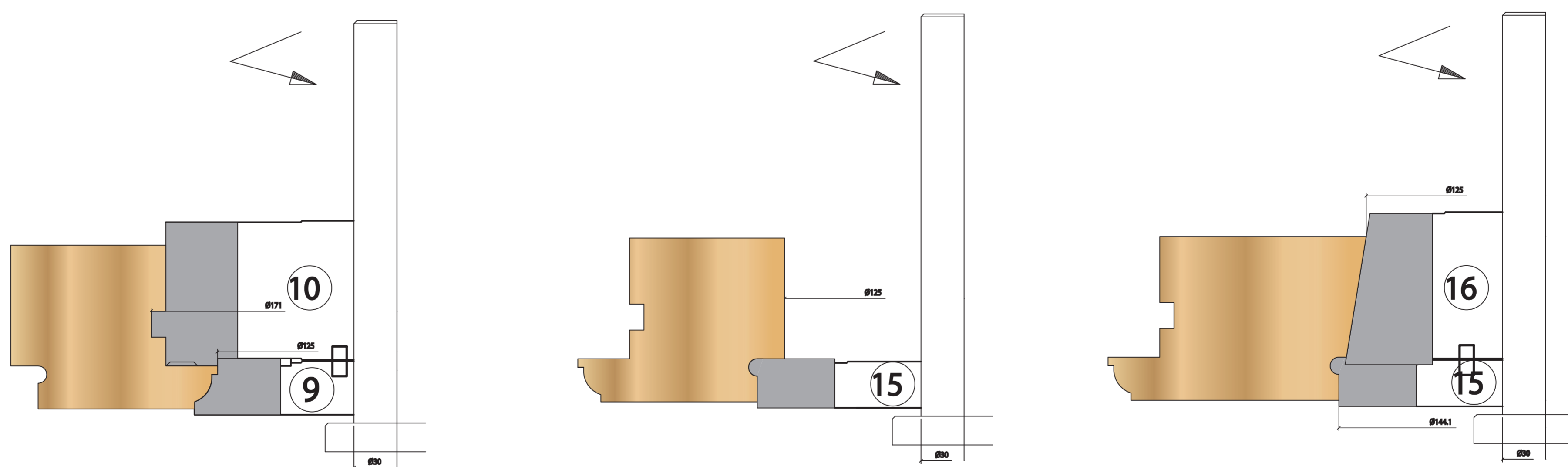
Casement Sash Profile
