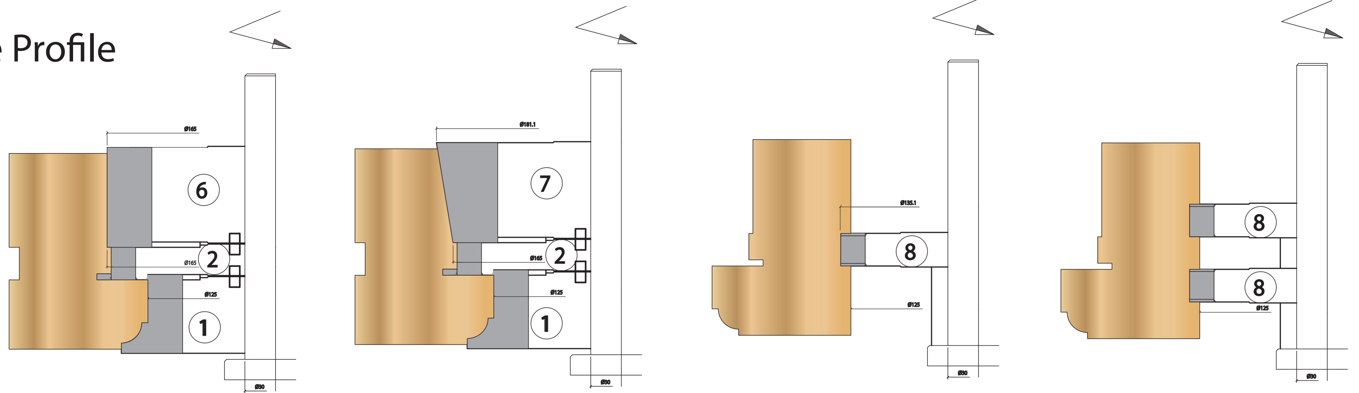
Tenon Frame
