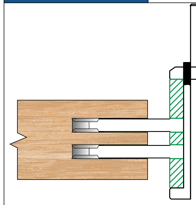
Sash Combe Slots
