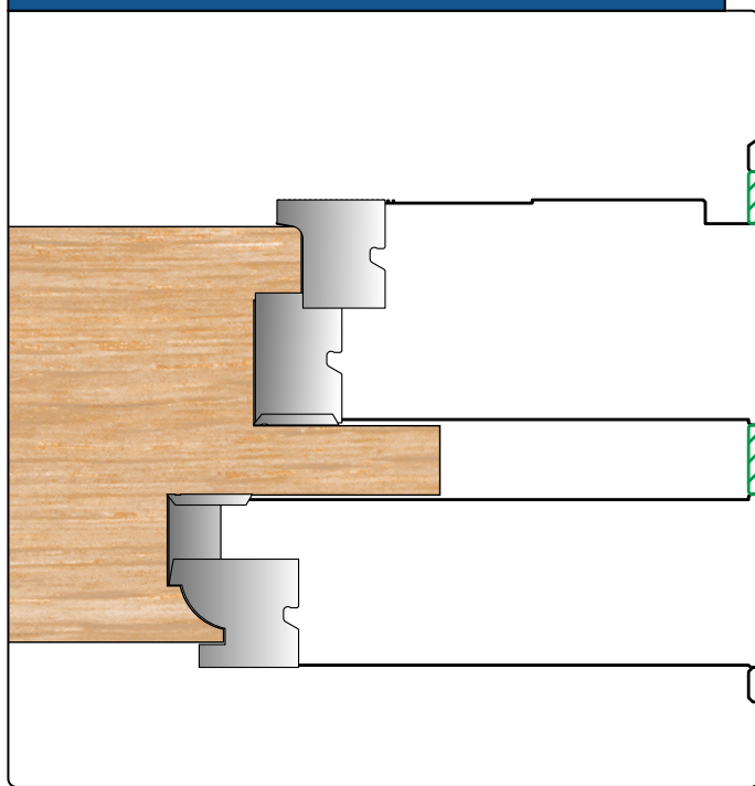
Frame Single Tenon Scribe
