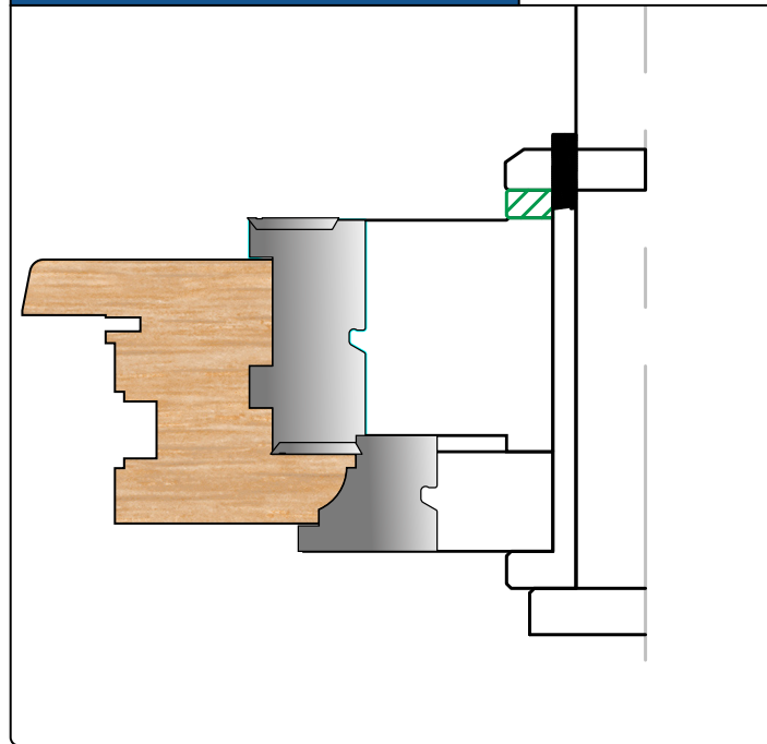
Inside Sash Mould
