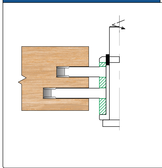
Frame Combe Joint Tenon Slots
