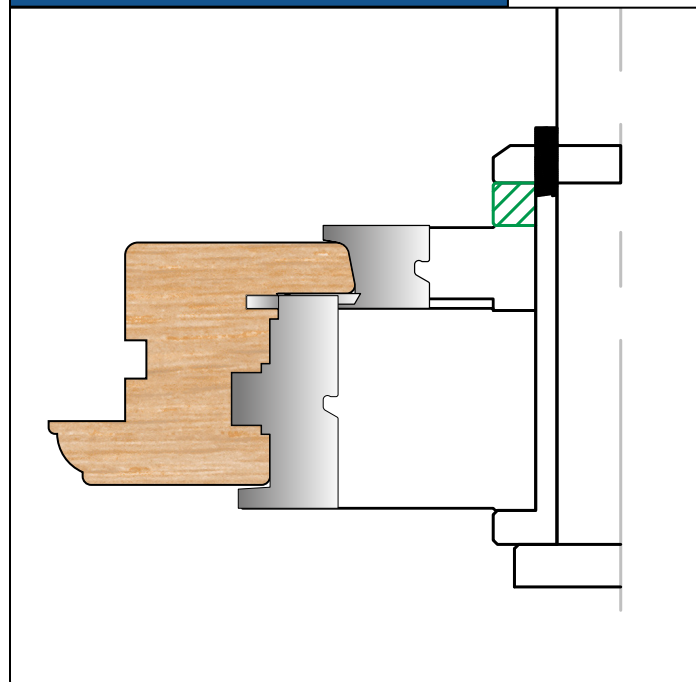
Outside Sash Mould
