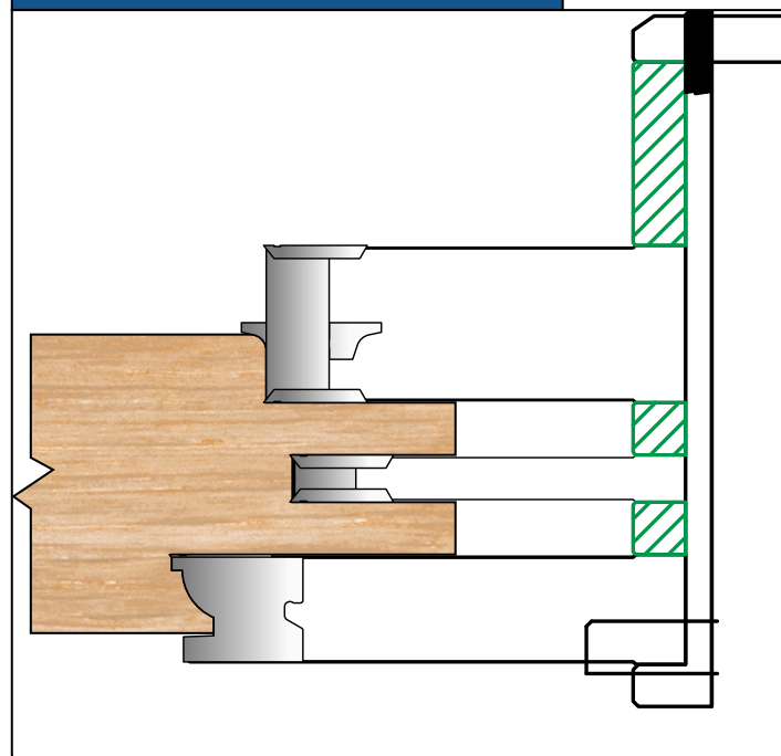
Sash Combe Mould
