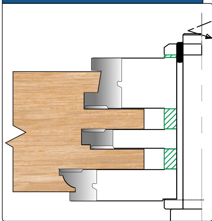
Frame Combe Joint Scribe Cill
