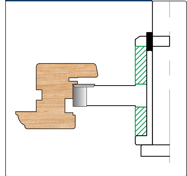
Sash Top/Bottom Rail
