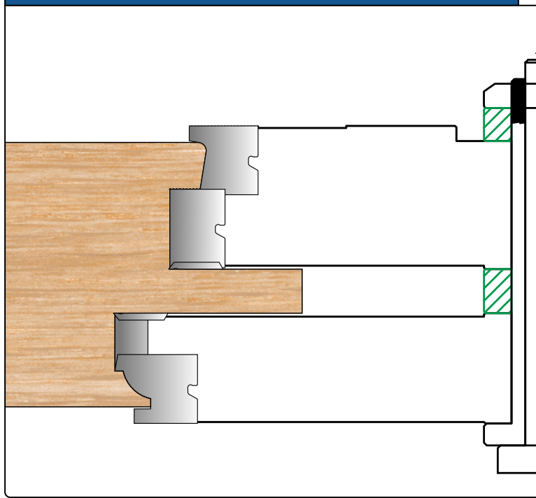
Frame Single Tenon Scribe Cill
