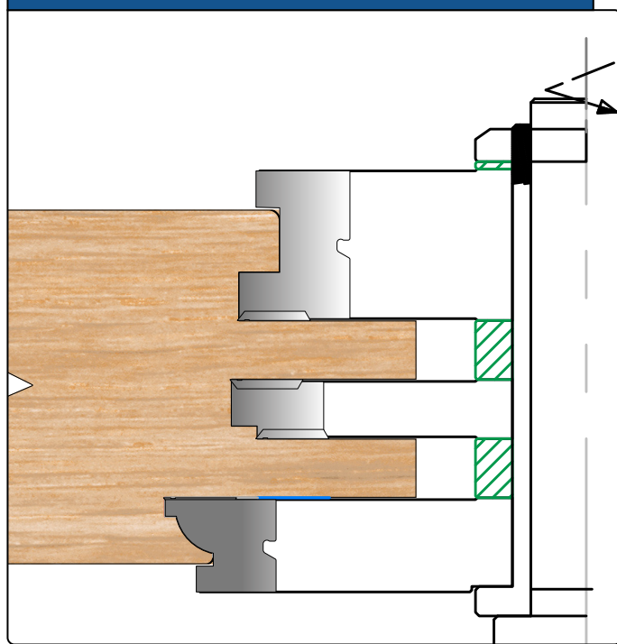
Frame Combe Joint Scribe
