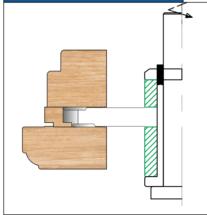
Frame Single Tenon Slot
