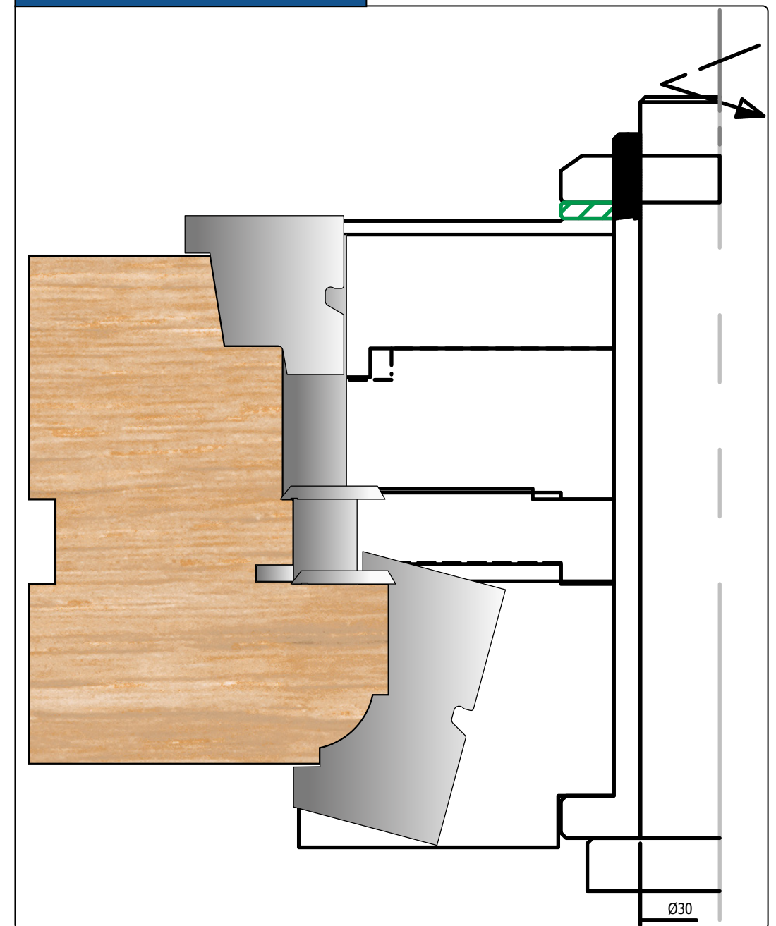
Frame Mould Cill
